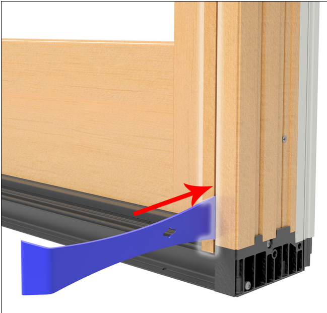
Figure 17 Remove interior side jamb parting stop.
