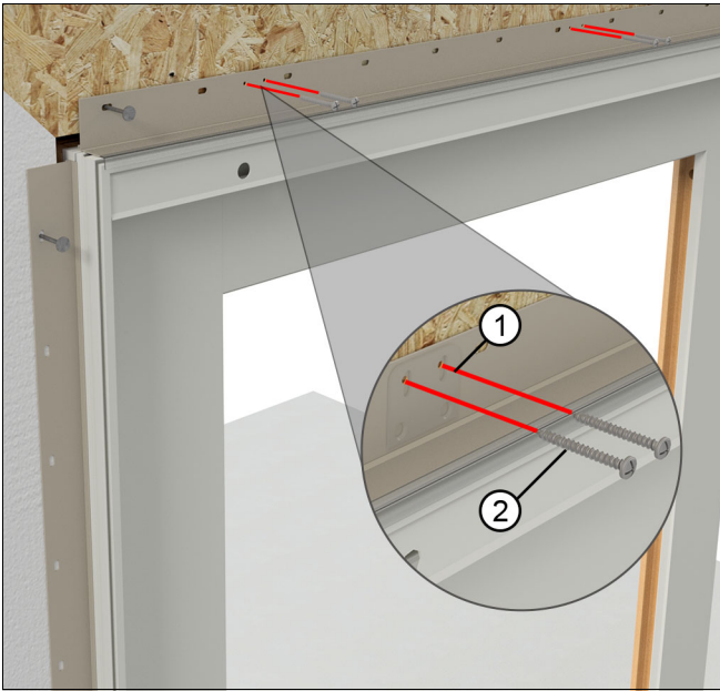
Figure 30 Fasten head jamb brackets to RO
