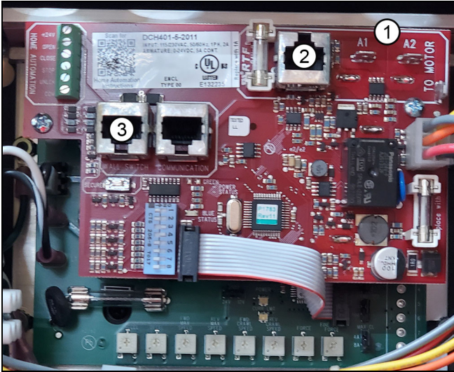
Figure 13 Control Box connections.
