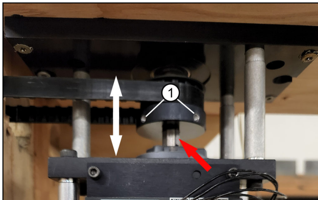
Figure 9 Drive pulley shown with belt attached
