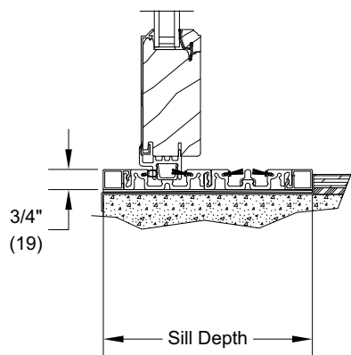
Flush Sill
