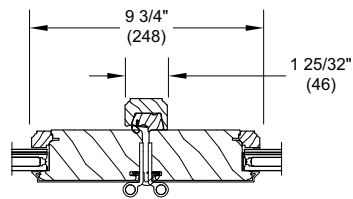
Astragal Detail with Ogee Sticking
