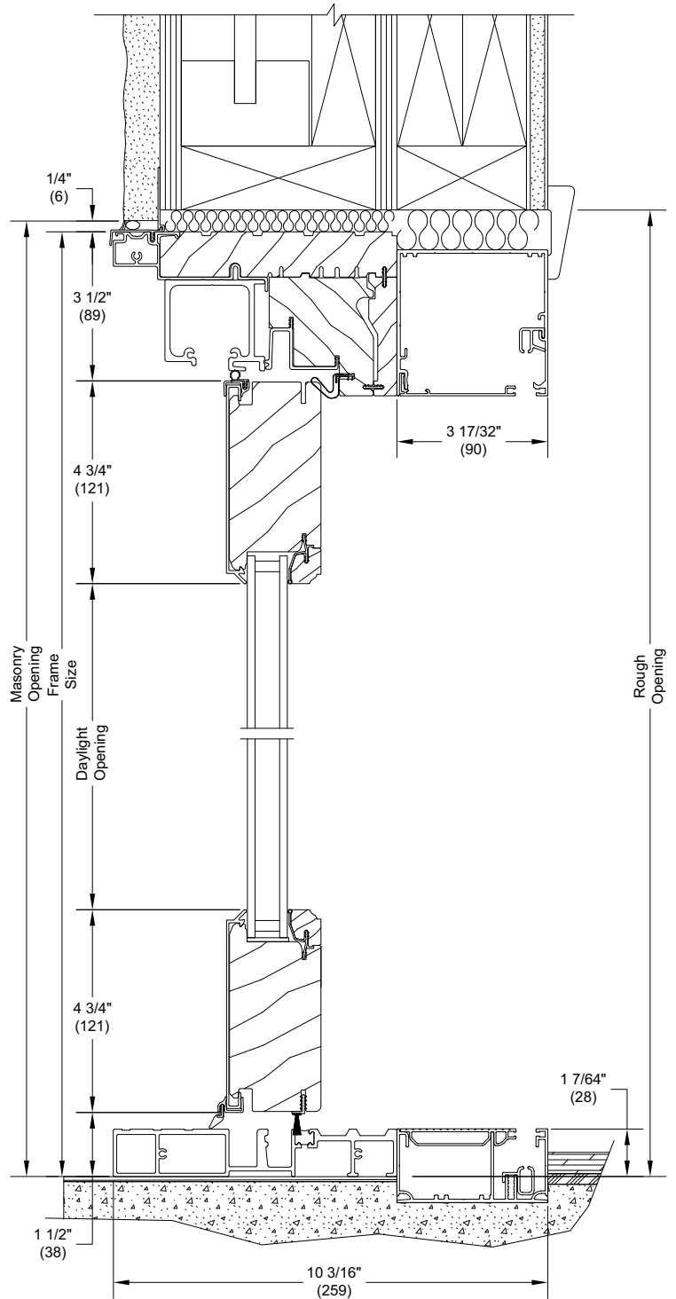
Head Jamb and Sill With Screen
