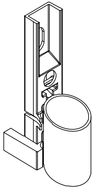
Interlock Seal, Sub Assembly
