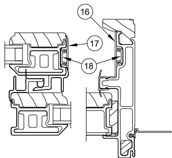
Stile and Jamb Covers Interior Painted Units Only
