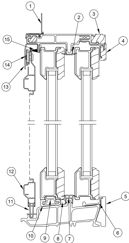
Head Jamb and Sill
