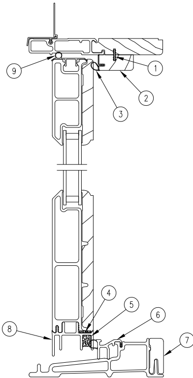
Head Jamb and Sill Detail
