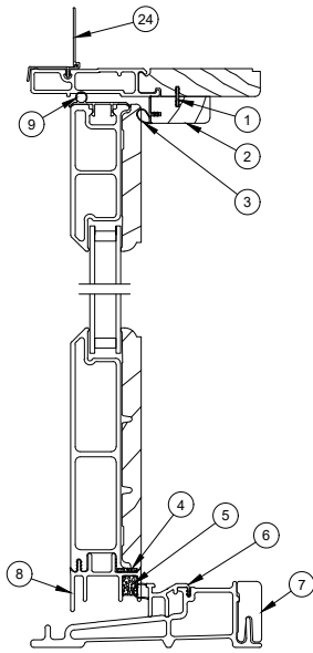
Head Jamb and Sill Detail
