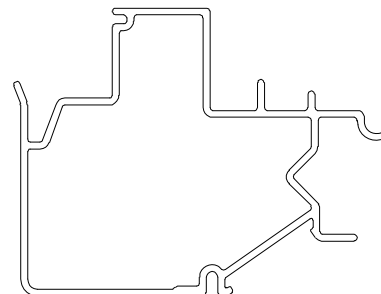
A3313 Pocket Interlock Support Block
