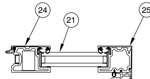
Bi-Parting Panel 1 1/4" Glass Jamb
