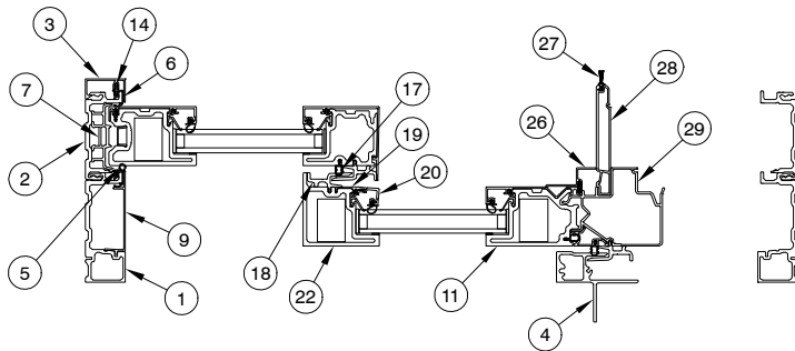
Pocket Uni-Directional Panel 15/16" Glass Jamb
