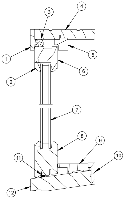
Head Jamb and Sill Detail
