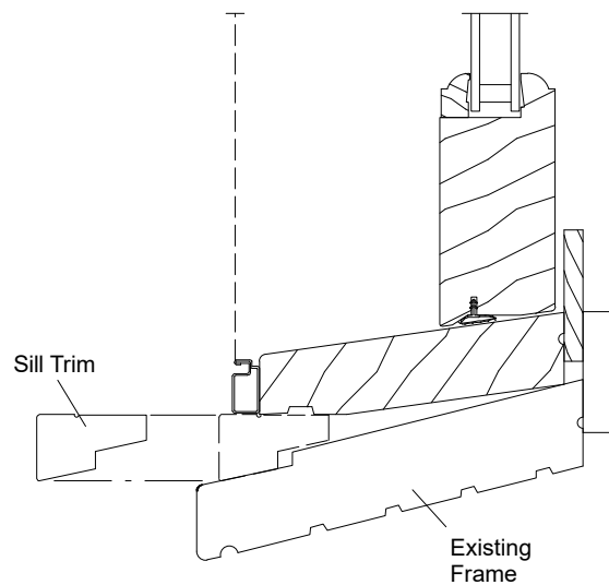
Sill Trim
