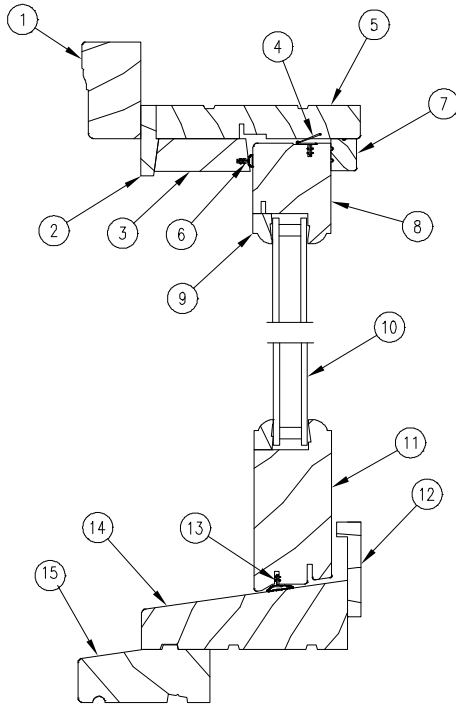
Head Jamb and Sill Detail
