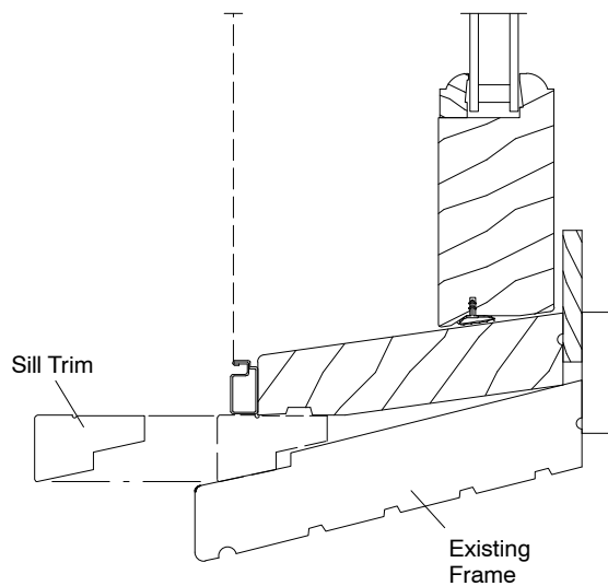
Sill Trim
