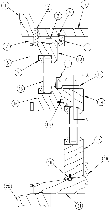
Head Jamb and Sill Detail
