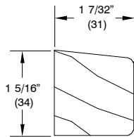
W12059 – Sill Nosing Transom
