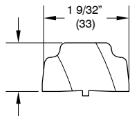
W10861 Mull Cover (Astragal)
