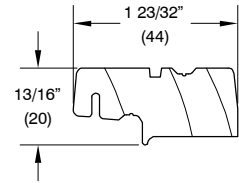
W10860 Mulling Cover Base (Astragal)
