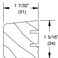
W8653 – Sill Nosing Transom – Pre-June 24, 2013
