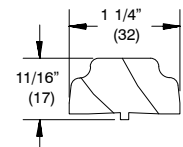
W7554 Astragal Cover and Transom Mull Cover – Wood
