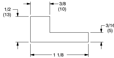
W7235* – Stationary Jamb Filler (Multi-panel)
