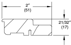
W8462 CMRT/Poly Stat Sash Stop, IZ4
