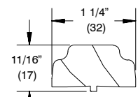
W7554 Astragal Cover
