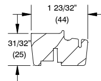
W9019 Mull Casing Base 71520469 – 6/8 Height 71520481 – 8/0 Height
