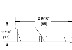
W7534 – Center Jamb Cover
