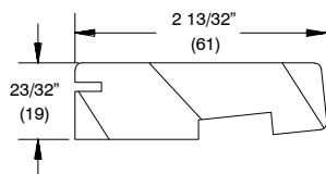
W6535 Head Jamb and Jamb Parting Stop
