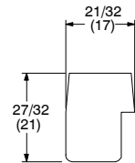
W7279 Operating Panel Track
