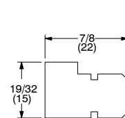
W7280 Head Jamb and Jamb Parting Stop
