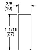
W7274 Head Jamb Liner and Stationary Jamb Liner
