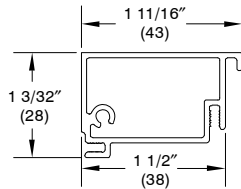
1 1/2" Flat Casing, A3069 200" (5080)
