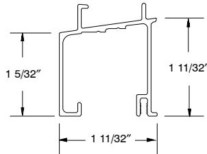
Simulated Thick Sill, A217 200" (5080)
