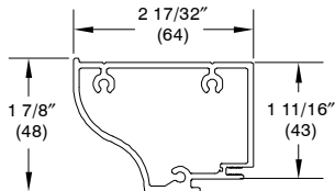
Thorton Enclosed Casing, A1909 200" (5080)
