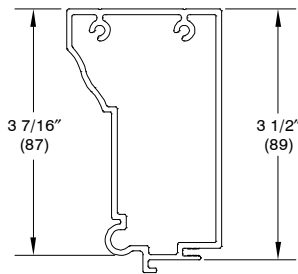
Columbus Casing, A1440 200" (5080)
