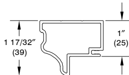
Potter Trim Casing, A1445 200" (5080)
