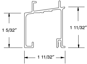
Simulated Thick Sill, A217 200" (5080)
