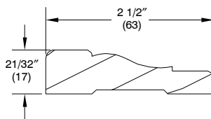
W1351, WM351 Interior Casing
