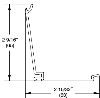
Subsill Lineal Cap, A1460 For A1452 Subsill 200" (5080)
