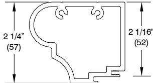
Stratton Enclosed Casing, A2366 200" (5080)
