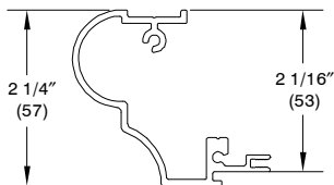
Stratton Casing, A1449 200" (5080)
