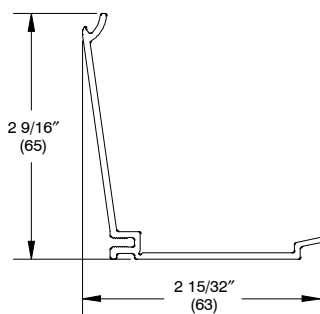
Subsill Lineal Cap, A1460 For A1452 Subsill 200" (5080)
