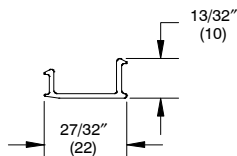
Subsill Lineal Cap, A1462 For A217 Subsill 200" (5080)
