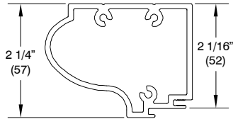
Ridgeland Enclosed Casing, A2881 200" (5080)
