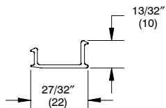
Subsill Lineal Cap, A1462 For A217 Subsill 200" (5080)
