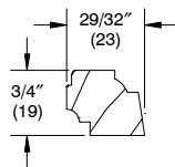
W4019 – Glazing Cap
