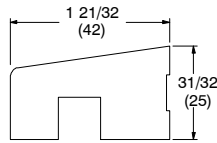
W7178 – Half Screen Nosing (WMSH)
