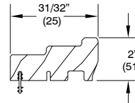
W8460 – Side Stop (replaces V1162)
