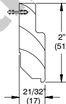
W7015 – Jamb Stop Stationary and Picture Units
