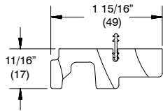
W8461 – Head Jamb Stop Operator
