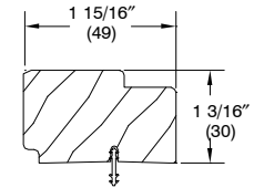
W8723 – Stationary Hardware Cover
