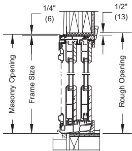
Head Jamb and Sill
