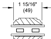
1 15/16" SDL W/Two Spacer Bar
