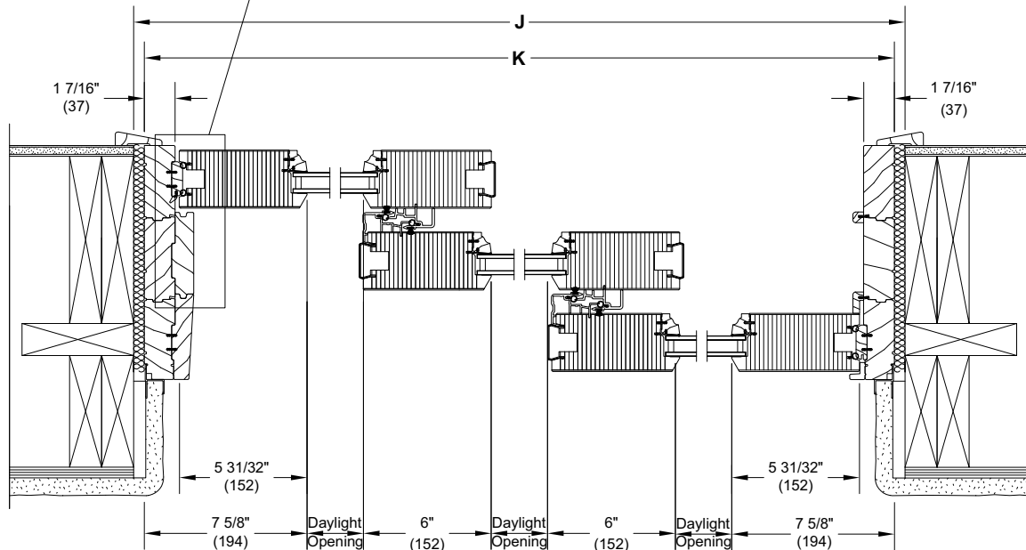
UWLSD STK - Tall Bottom Rail Uni-Directional - XXO
