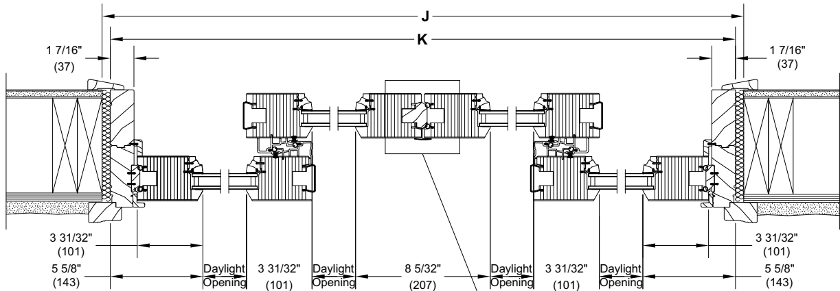
UWLSD STK - Short Bottom Rail Bi-Parting OX-XO
