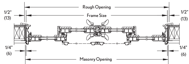
4 Panel Jamb - OXXO Operator size <= 86"
