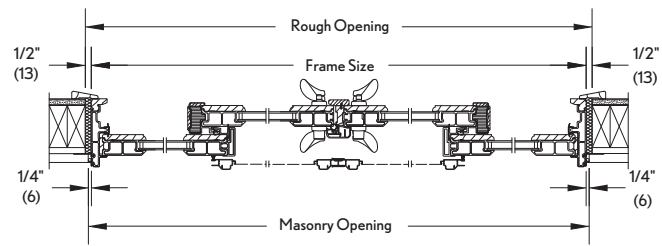
4 Panel Jamb - OXXO Operator size > 86"
