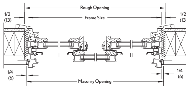
Triple Sash XOX Operator Jamb
