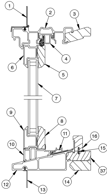
Head Jamb and Sill Stationary
