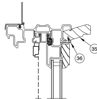
Head Jamb Interior Painted Units Only
