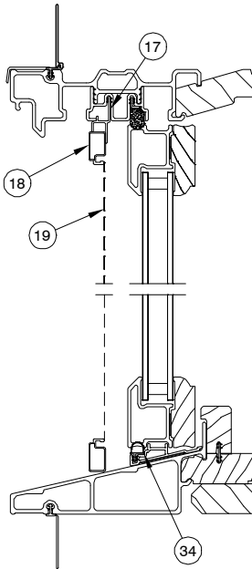
Head Jamb and Sill Operator
