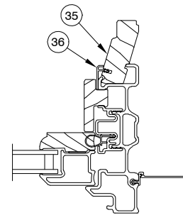
Jamb Interior Painted Units Only
