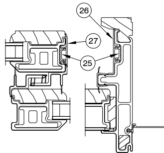
Stile and Jamb Covers (Painted Interior units only)
