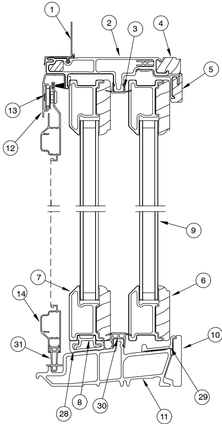
HEAD JAMB AND SILL DETAIL OPERATOR
