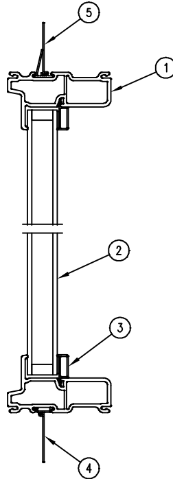
HEAD JAMB & SILL DETAIL
