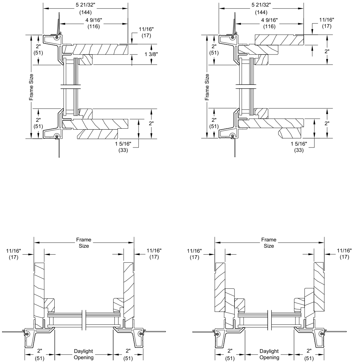
Double Hung
